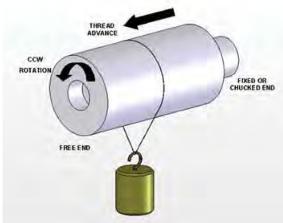
Figure 3 — Counter-Clockwise Lead
